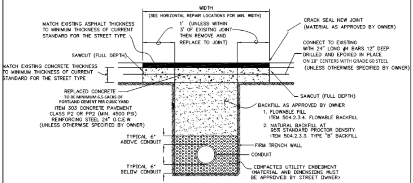
CONCRETE PAVEMENT WITH ASPHALT OVERLAY N.T.S.
