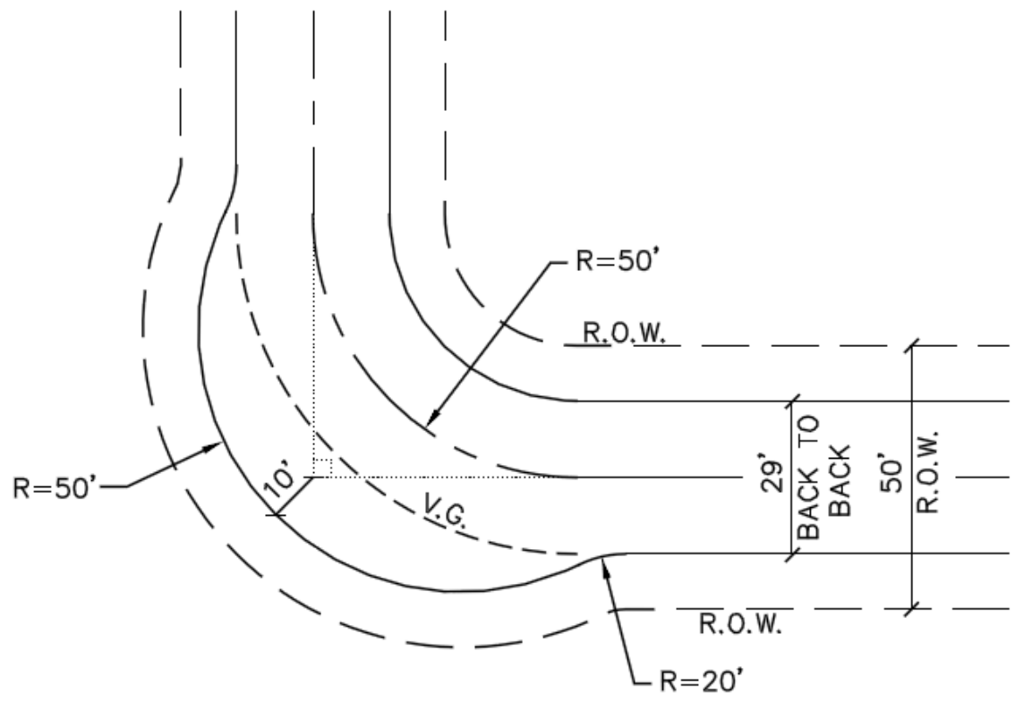
TYPICAL EYEBROW
