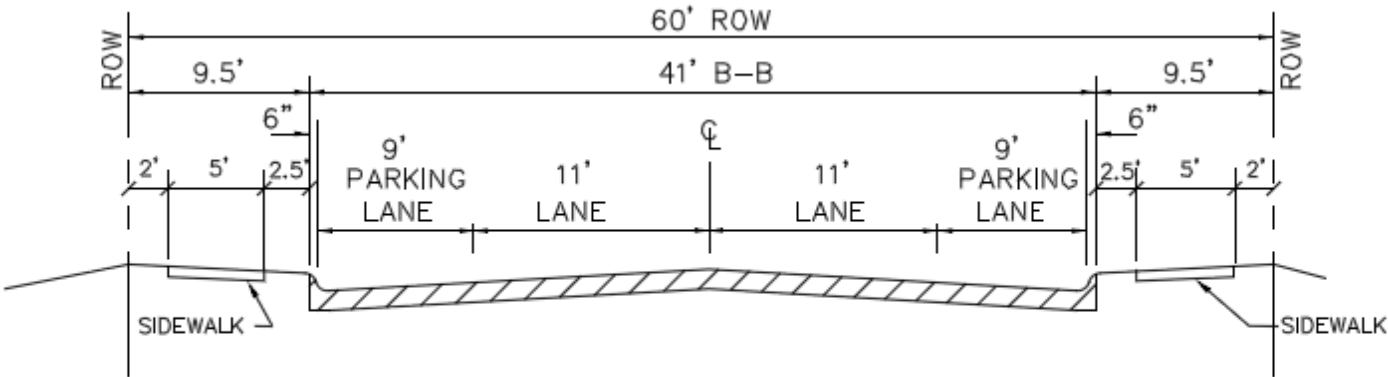
MINOR COLLECTOR AND/OR LOCAL COMMERCIAL UNDIVIDED
