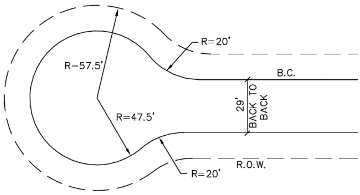
TYPICAL CUL-DE-SAC
